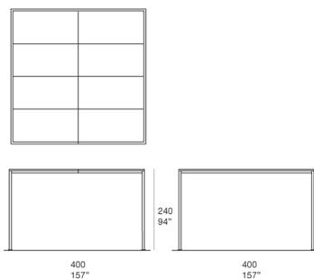
CA01A - CA01AH senza base / without base
