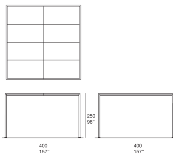
CA01AB - CA01ABH con base / with base
